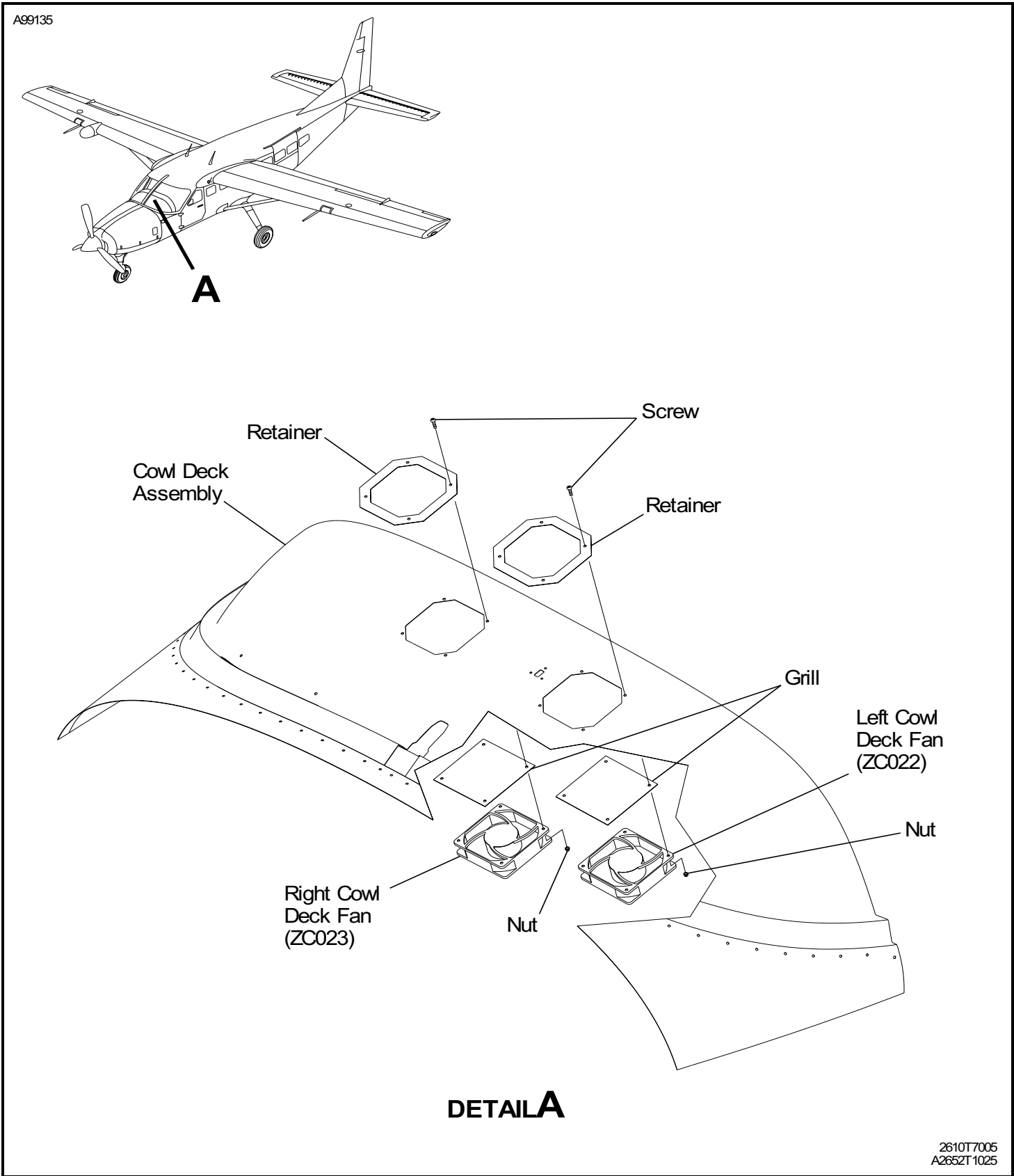
Figure 401 : Sheet 1 : Cowl Deck Cooling Fan Installation
